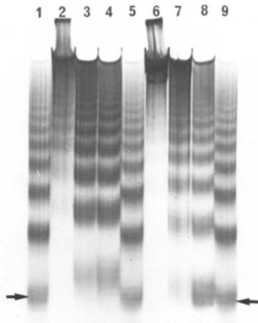
Fig.1. Polyacrylamide gel electrophoresis of the DNA of micrococcal nuclease digests of chromatin from sea urchin sperm cells (slots 2–4), sea urchin embryo cells at the gastrula stage (slots 6–8) and rat liver (slots 1, 5, 9). Nuclease digestions of sperm and gastrula chromatin were carried out for increasing times of digestion as described in Materials and methods. The arrows point to the position of the rat liver monomer DNA fragment.
